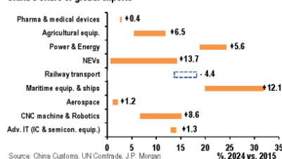
China's share of global exports
